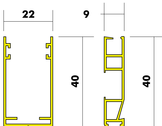
Left: Dimensions of Cassette Case, Side Guides & Bottom Bar.
